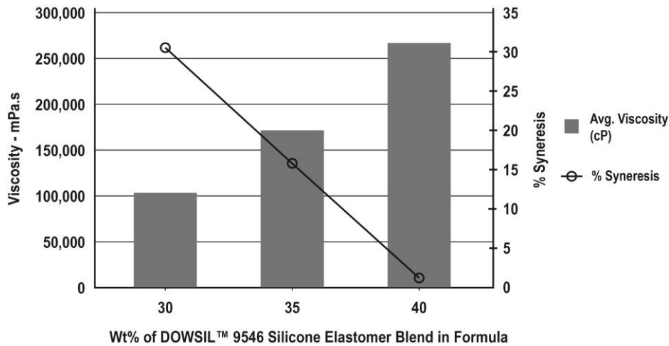
Figure 6: In soft solid applications, DOWSIL™ 9546 Silicone Elastomer Blend significantly reduces syneresis.
